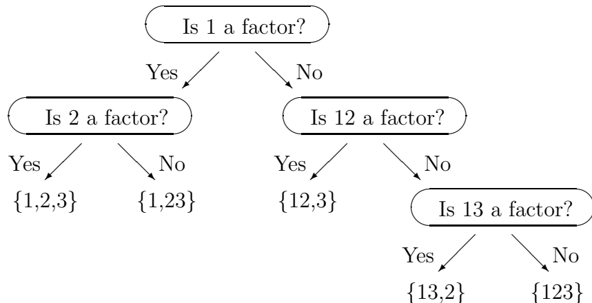
Fig. 1. Illustration of the combinatorial method to factor a cubic, given by witness points 1, 2, 3. Every question is answered by a linear trace test.
